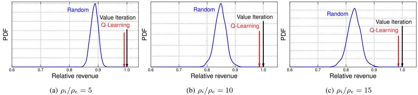
Fig. 6: The distribution of the revenues obtained by random smart policies compared to the proposed algorithms.
